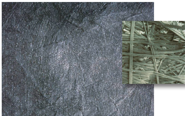
Figure 15. Non-woven heat bonded geotextile with close-up
