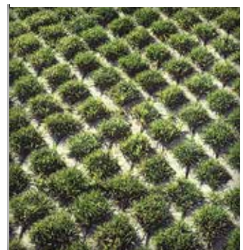
Figure 2. A typical grid pavement for occasional vehicular traffic
