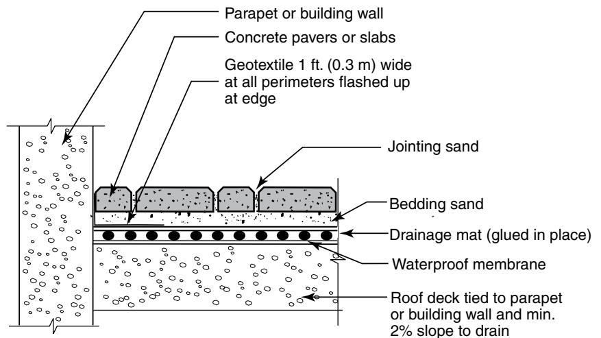
Figure 11. Detail showing geotextile at all edges of sand and aggregate bedding courses for a pedestrian application.
