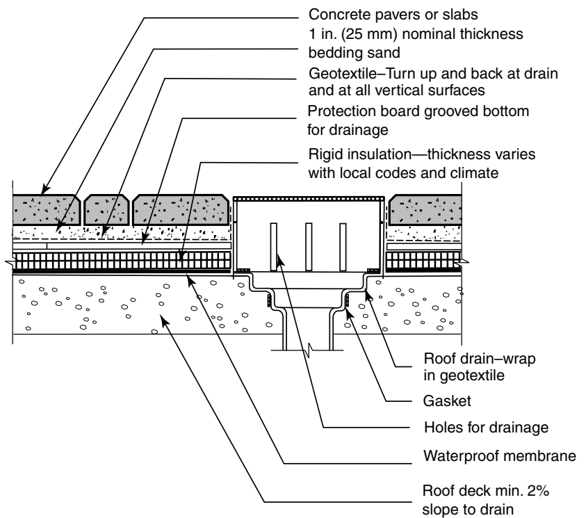
Figure 17. A bi-level drain detail for a pedestrian plaza deck over habitable space.
